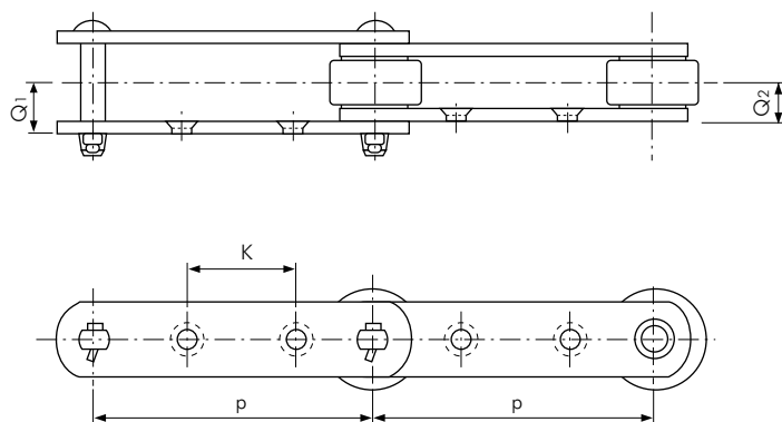
GA-2 Attachment
