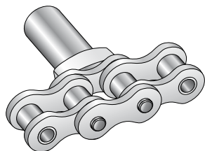
Fig. 25 Extended Pin Attachments with Jigs
