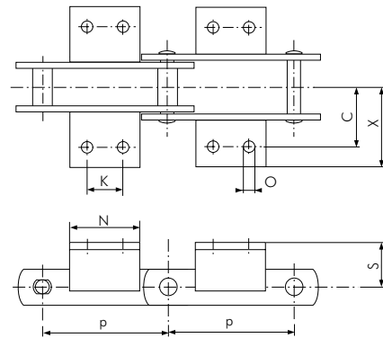
K-2 Attachment
