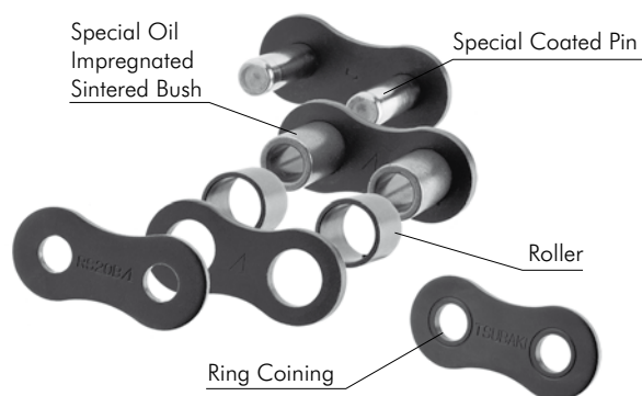
Fig. 31 Basic Construction
