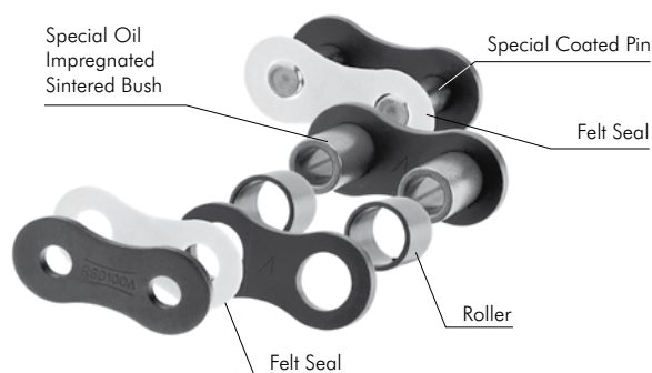
Fig. 10 Basic Construction
