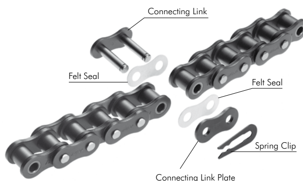
Fig. 11 Connecting Method ANSI X-LAMBDA
