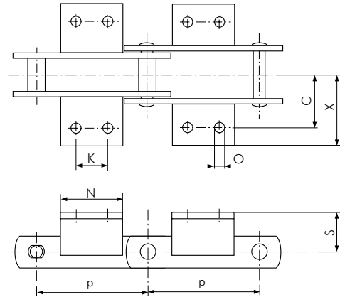
K-2 Attachment
