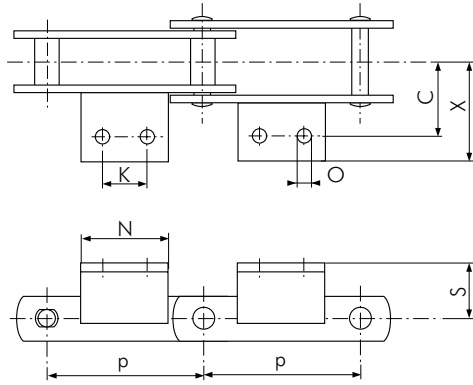
A-2 Attachment
